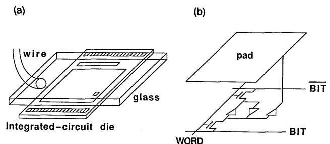
Fig. 1. (a) Construction of the FLC/silicon IC SLM. (b) Schematic diagram of the SLM square-array SRAM element. The element's state is changeable only when the WORD line is high; otherwise the static latch formed by the cross-coupled inverters holds the state last determined by the BIT and \overline{\text{BIT}} lines. The latch output is buffered by the third inverter onto the FLC driving pad.
