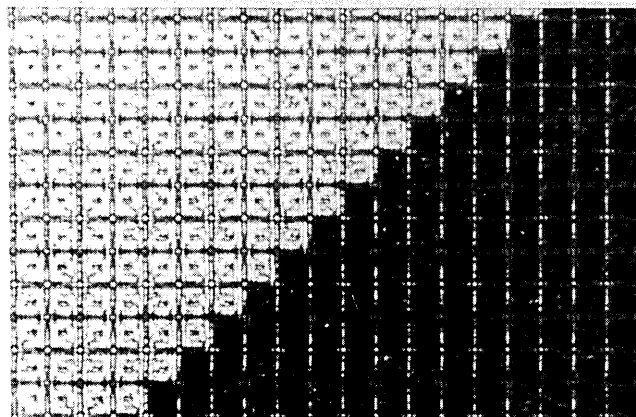
Fig. 2. Reflected light microphotograph of a portion of the 64 \times 64 square array between crossed polarizers. The array has been oriented so that the FLC state in half the elements has its optic axis parallel to the polarizer. These elements appear dark, while the other elements appear bright, their FLC axis making an angle \approx 25^\circ to the polarizer. The elements are on 60\text{-}\mu\text{m} centers.
