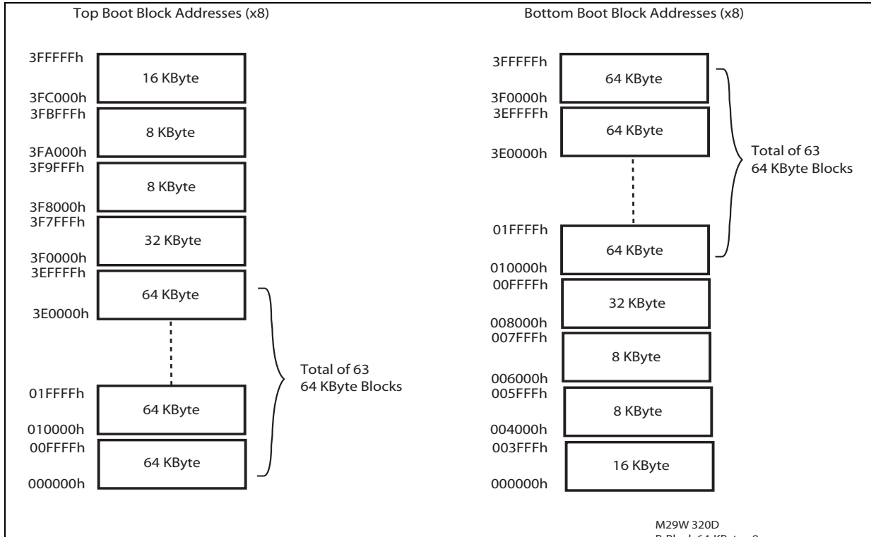
Figure 5. M29W320D block addresses (x8)
